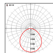
200W-5000K-120°
