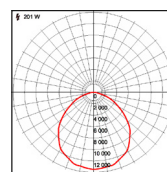
200W-5000K-90°
